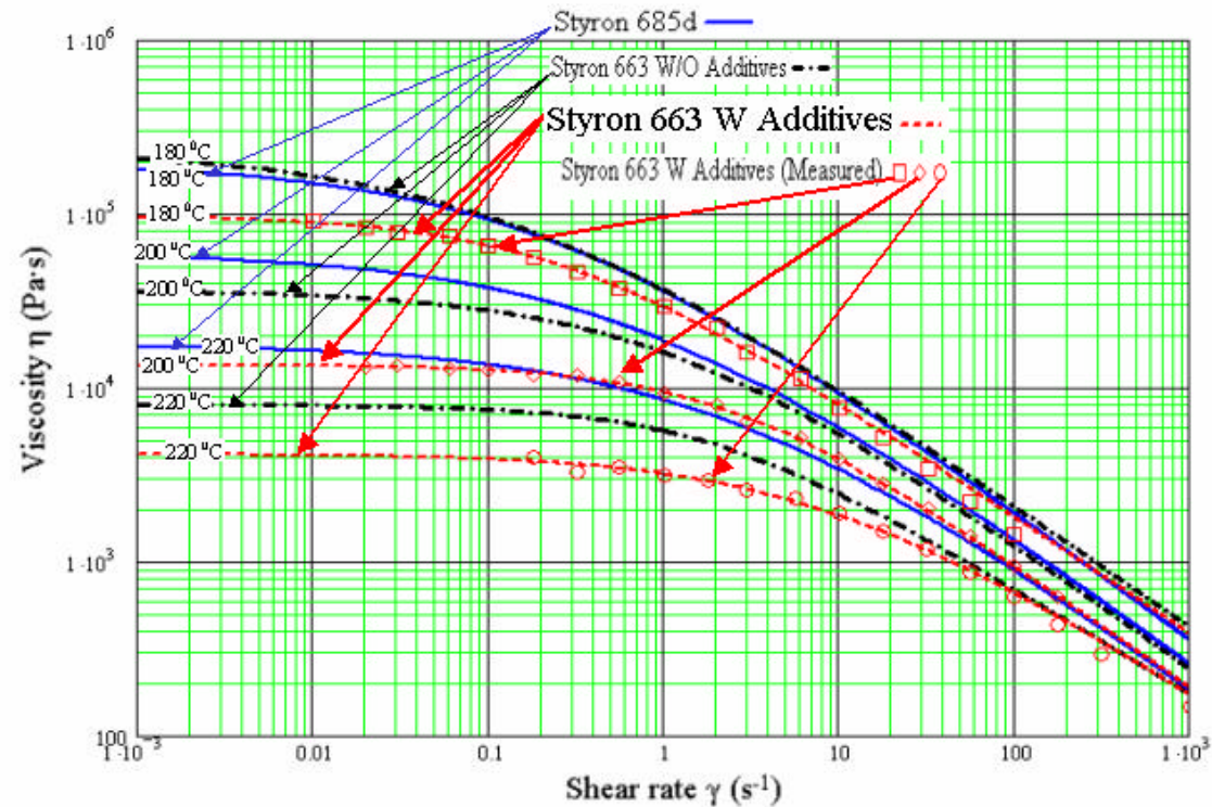
Figure 1: Plot of polymer viscosity as a function of shear rate and temperature
